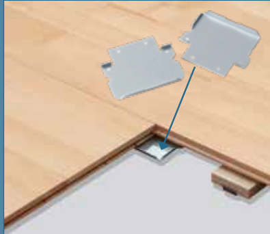
ASSEMBLY BRACKETS
